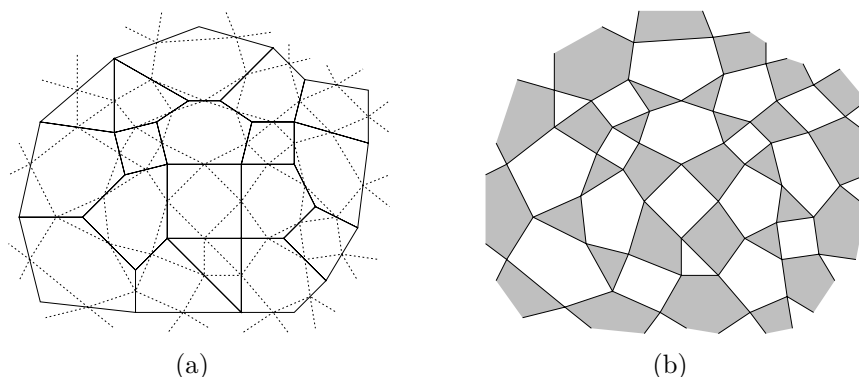
FIGURE 3. A cellular decomposition (a) and its medial decomposition (b)
