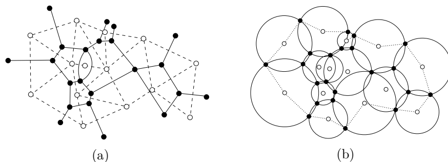
FIGURE 2. A cellular decomposition of the disc and a corresponding circle pattern with circles meeting at diverse angles
