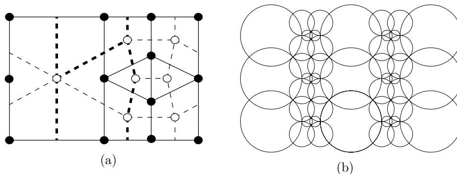
FIGURE 1. A cellular decomposition of the torus and the corresponding circle pattern with orthogonally intersecting circles
