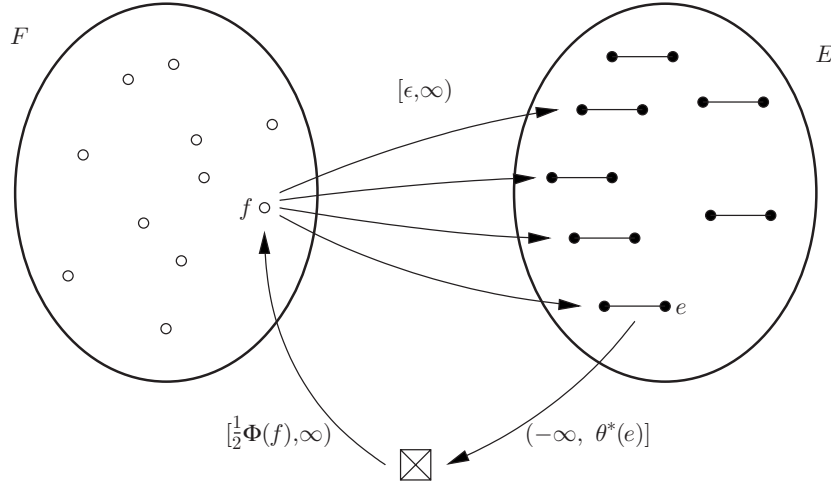
FIGURE 5. The network (N, X) . Only a few of the branches and capacity intervals are shown.
