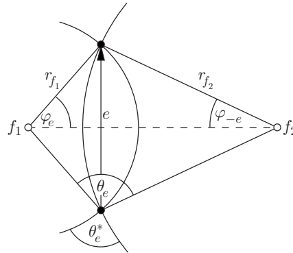
FIGURE 4. A Euclidean kite-shaped quadrilateral, \theta_e + \theta_e^* = \pi
