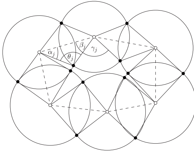
FIGURE 7. The circles and quadrilaterals corresponding to a simple closed copath after stereographic projection
