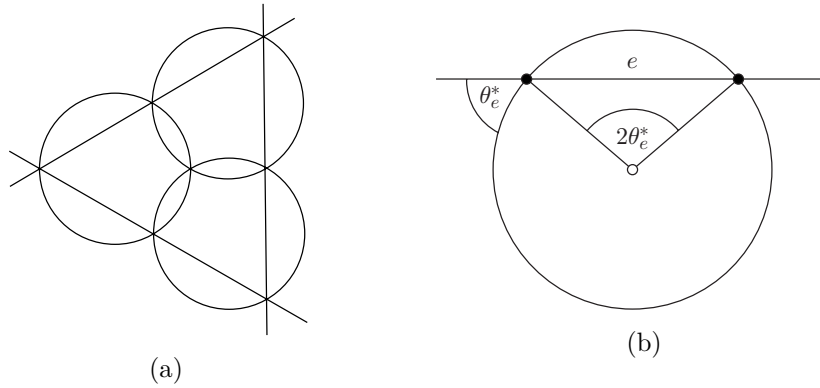
FIGURE 6. (a) The regular cubical pattern after stereographic projection. (b) How to calculate the \Phi_f for the new boundary circles.
