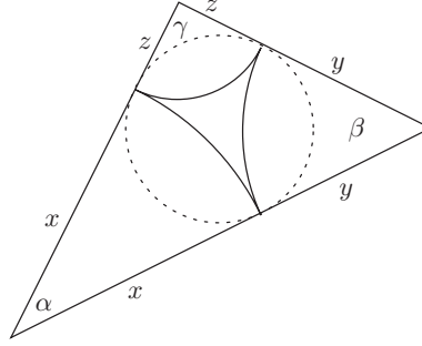
FIGURE 8. A Euclidean triangle
